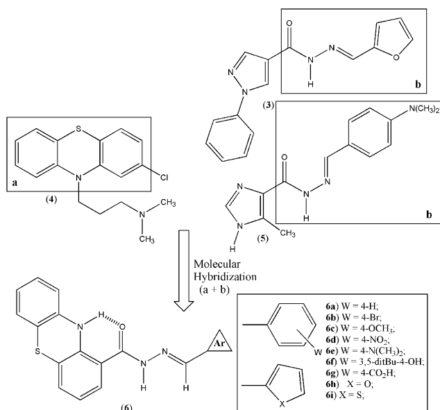
Figure 2. Design concept of new 10 H -phenothiazine-1-acylhydrazone derivatives ( 6a–i ).
