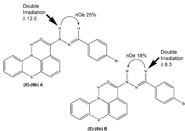
Figure 3. NOE correlations between carbonyl N–H bond and benzylidene hydrogen of the para -bromo derivative ( 6b ).
