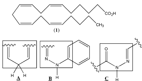
Figure 1. Hydrazone (B) and acylhydrazone (C) groups as mimicks of bis-allyl fragment (A) of arachidonic acid (I).
