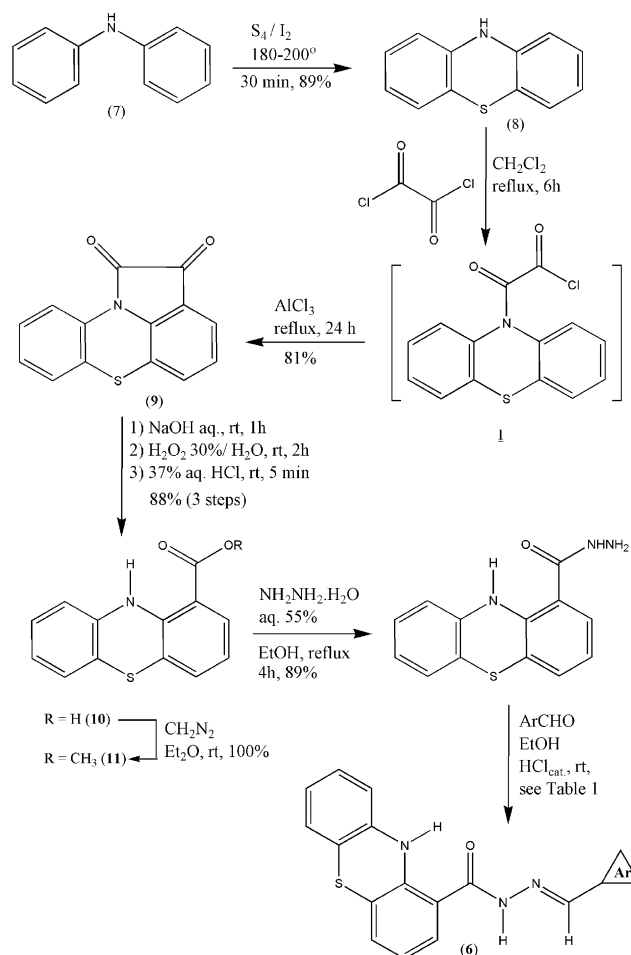
Scheme 1. Synthetic route for the preparation of phenothiazine NAH derivatives ( 6a–i ).
